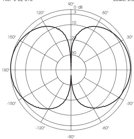
TYPICAL RADIATION PATTERN in E-plane at 222 MHz TYPICAL RADIATION PATTERN in E-plane at 258 MHz File: E-02-015 Scale: linear File: E-02-016 Scale: linear
