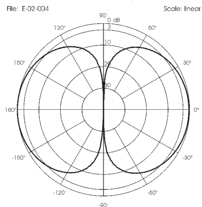
TYPICAL RADIATION PATTERN in E-plane at 135 MHz
