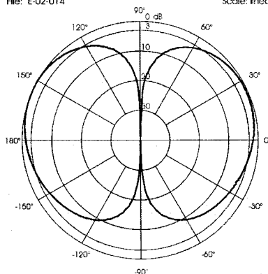
TYPICAL RADIATION PATTERN In E-plane at 145 MHz File: E-02-014 Scale: linear
